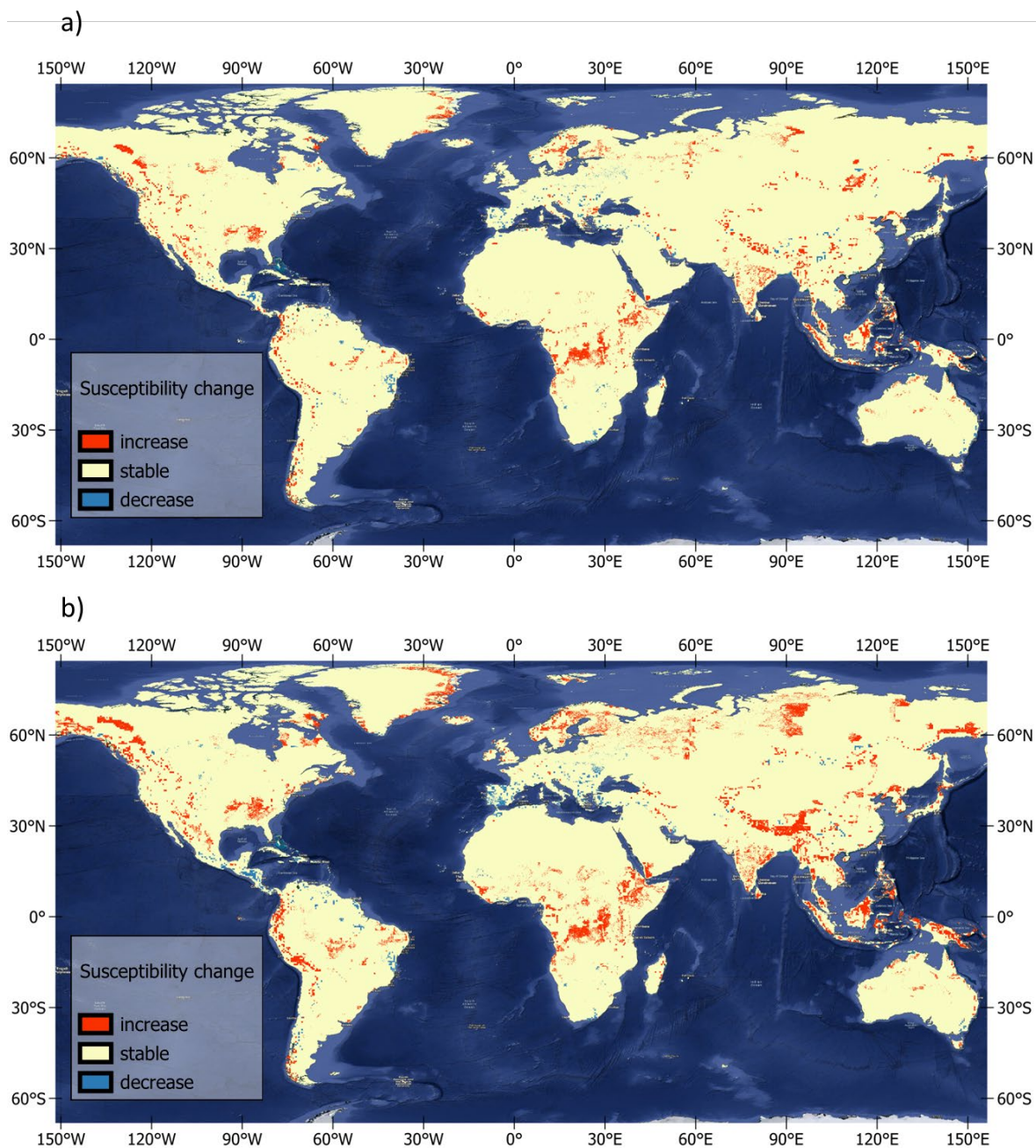
Figure 8 (a) Difference between the susceptibility map for rainfall-induced landslides with today's climate and the susceptibility map for the future climate assuming an SSP126 scenario. (b) Difference between the susceptibility map for today's climate and future climate assuming an SSP585 scenario.
