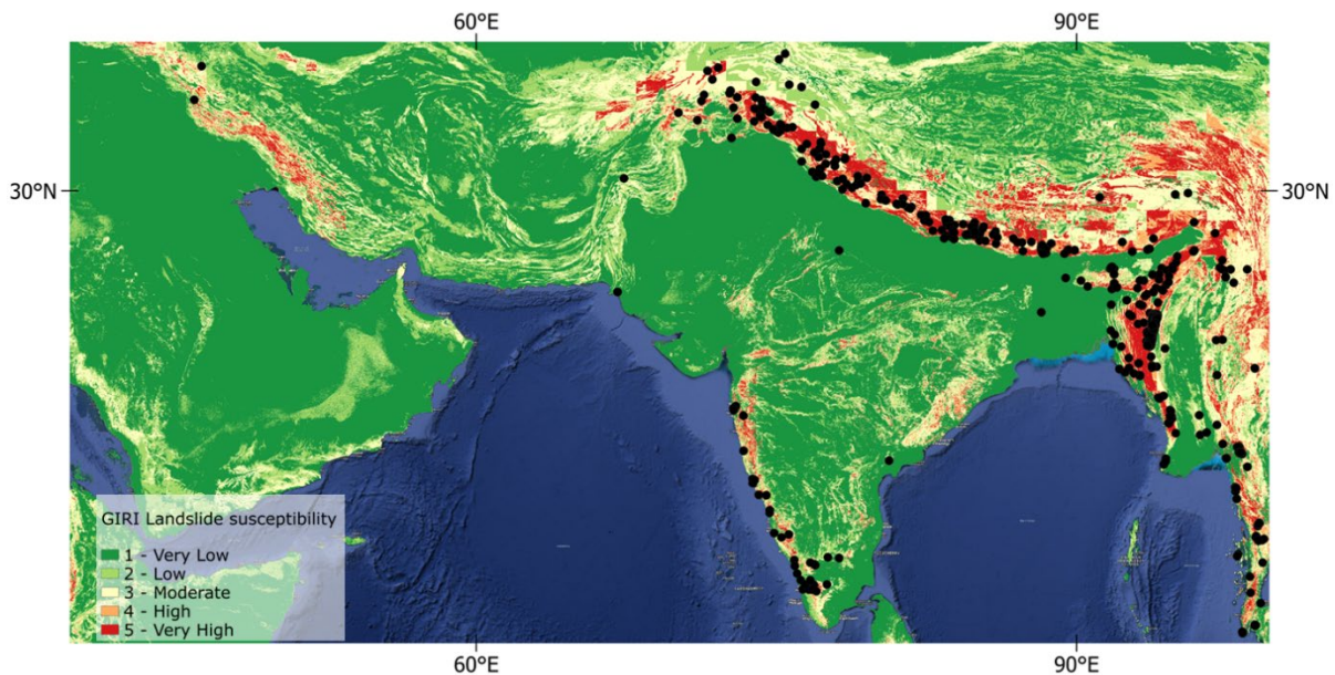
Figure 7 Susceptibility to rainfall-induced landslides obtained with the GIRI model for current climate conditions over Southeast Asia. The Black points represent the Landslides in the NASA COOLR database (Kirschbaum et al. 2010; Juang et al. 2019).
