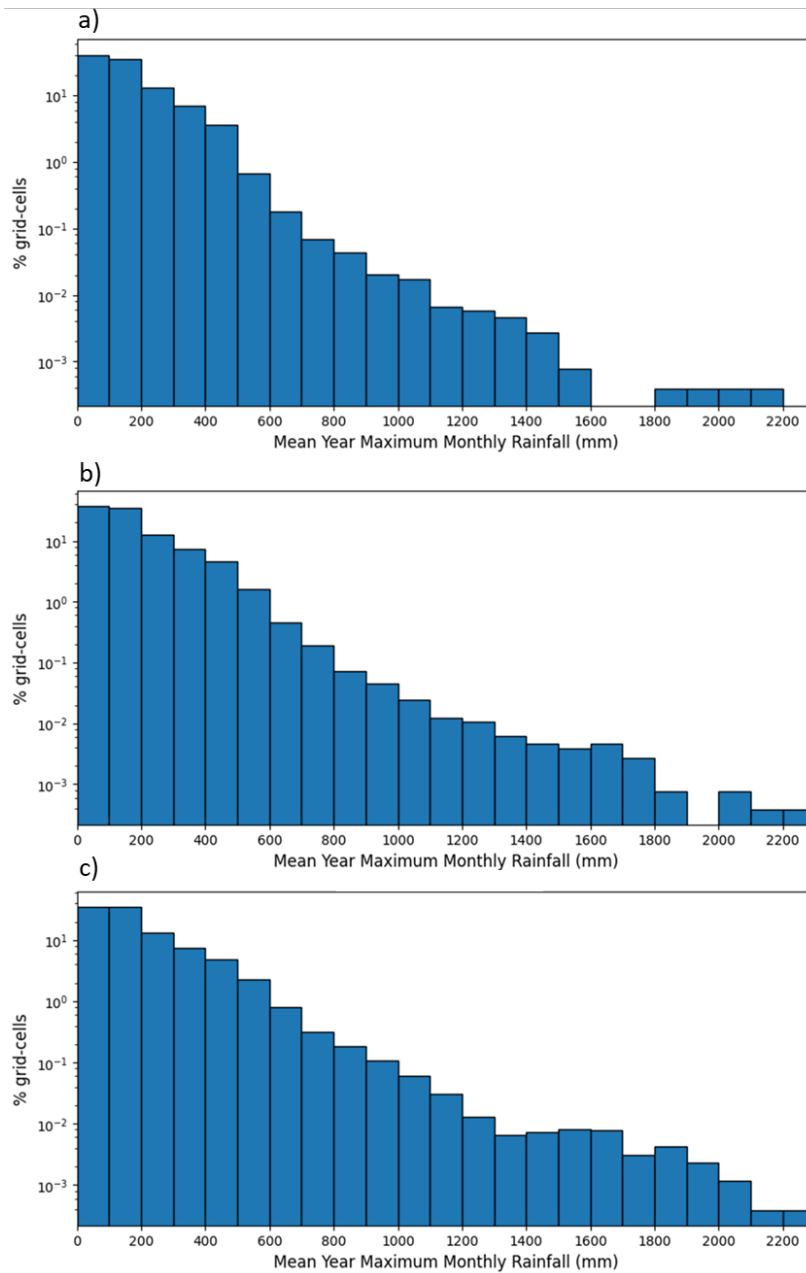
Figure 2 Mean year maximum monthly precipitation in (a) current climate conditions and in the period 2061-2100 with the (b) SSP126 and (c) SSP585 climate change scenarios.
