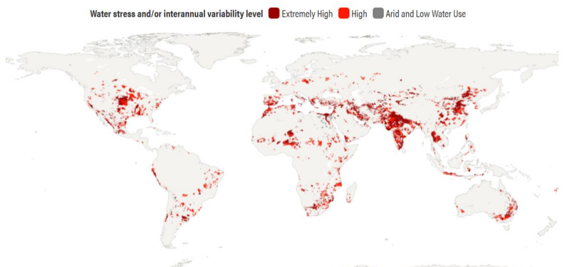
Figure 3.1. Global crop areas at high risk of water stress and/or variability
