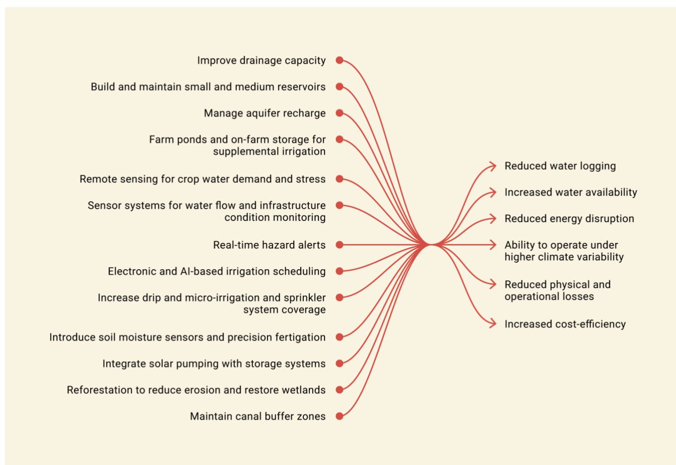
Figure 4.1. Technology investments in irrigation systems and resulting resilience benefits
