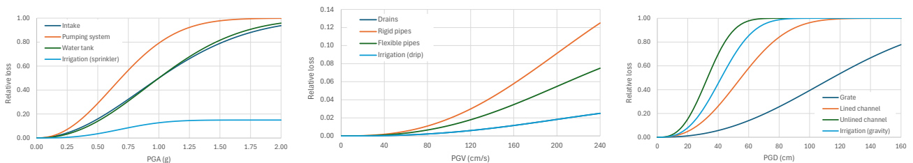
Figure 2.6. Vulnerability functions for irrigation system elements for earthquakes
