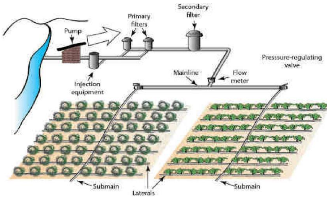
Figure 2.5. Main components of a drip irrigation system
