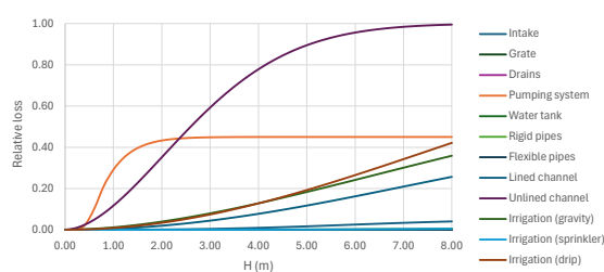
Figure 2.7. Vulnerability functions for irrigation system elements for floods
